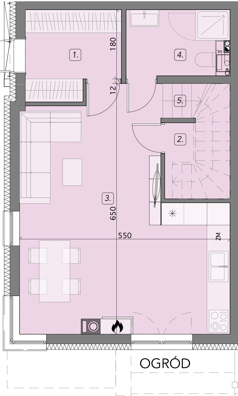
PARTER
